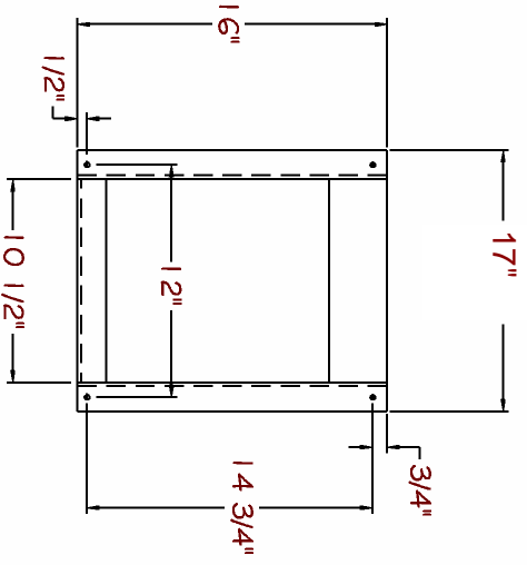
Front Box Mtg. Frame
